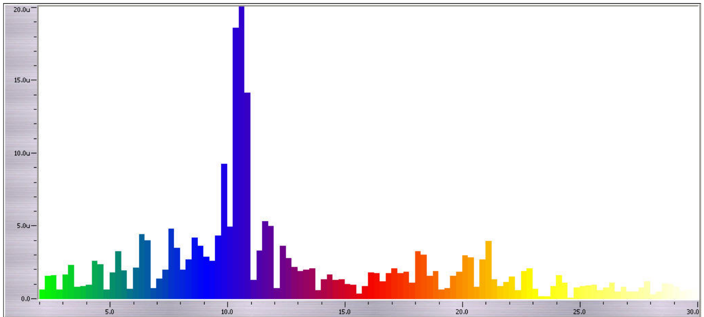
Figure 5: Spectral analysis of EEG in figure 1. Note the high peak around 10 Hz - this corresponds to the alpha rhythm.
