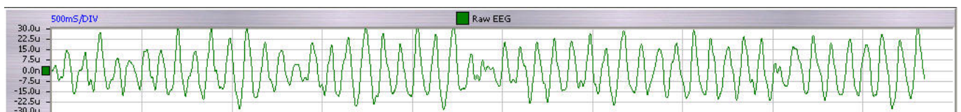
Figure 1: a relatively rhythmic EEG. Though the amplitude (vertical axis) varies, the duration (horizontal axis) of each cycle is stable, at around 1 cycle per 0.1 seconds - a frequency of around 10 Hz.
