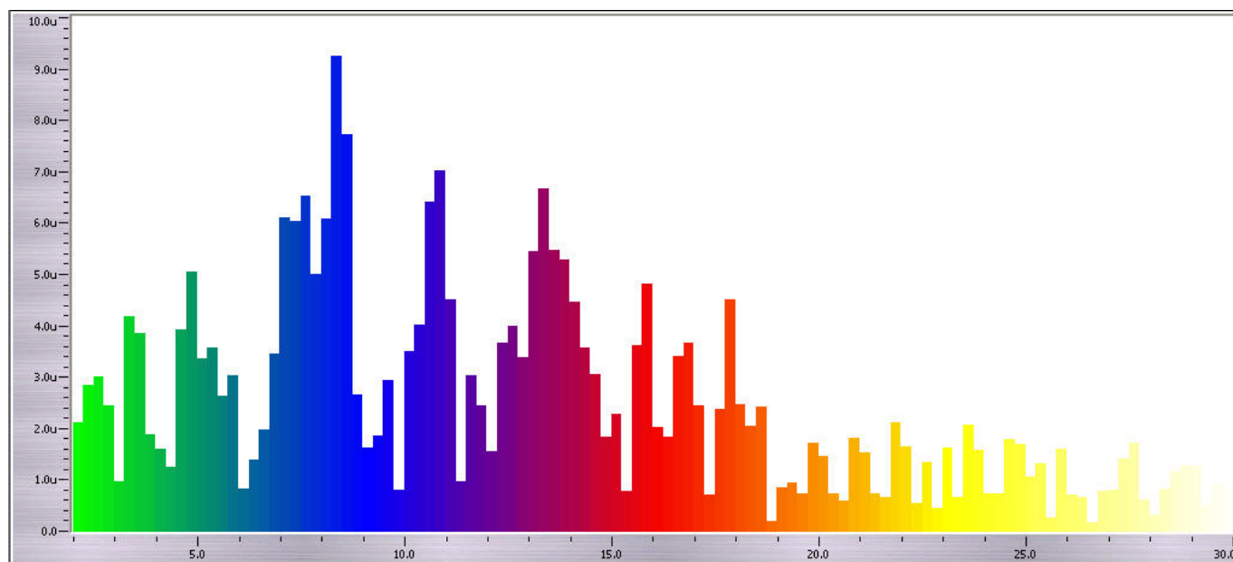
Figure 4: Spectral analysis of EEG shown in figure 2 - mixed frequencies.
