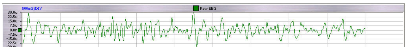
Figure 2: An EEG recording with no discernible rhythm.
