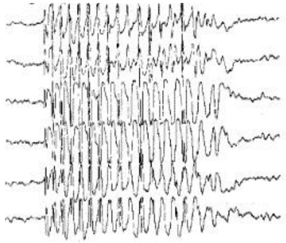
Figure 6: EEG during a brief epileptic seizure.
